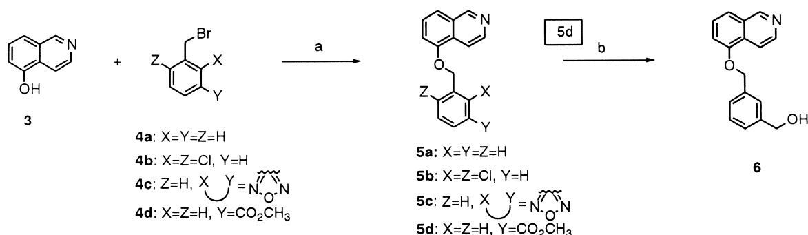
Scheme 1. Reagents: (a) NaH, DMF; (b) LAH, THF.
