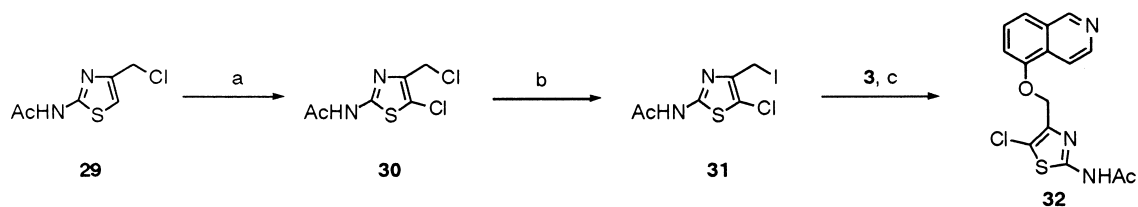
Scheme 6. Reagents: (a) NCS, \text{CHCl}_3 ; (b) \text{NaI} , acetone; (c) \text{NaH} , DMF.
