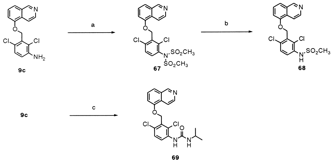
Scheme 11. Reagents: (a) \text{MsCl} , \text{Et}_3\text{N} , \text{CH}_2\text{Cl}_2 ; (b) 1 N-NaOH; (c) isopropyl isocyanate, \text{Et}_3\text{N} , EtOH.
