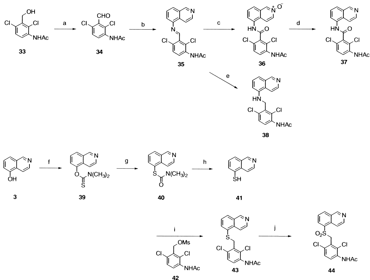
Scheme 7. Reagents: (a) \text{MnO}_2 , \text{CHCl}_3 ; (b) 5-aminoisoquinoline, EtOH; (c) mCPBA, \text{CHCl}_3 ; (d) 10% Pd-C, \text{NH}_4^+\text{HCO}_2^- , MeOH; (e) \text{NaBH}_4 , EtOH; (f) dimethylthiocarbamoyl chloride, NaH, DMF; (g) \Delta ; (h) 1 N -NaOH, MeOH; (i) \text{Et}_3\text{N} , DMF; (j) \text{KMnO}_4 , AcOH, \text{H}_2\text{O} .
